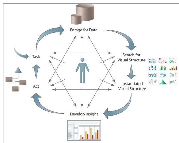
FIGURE V: Data Exploration
