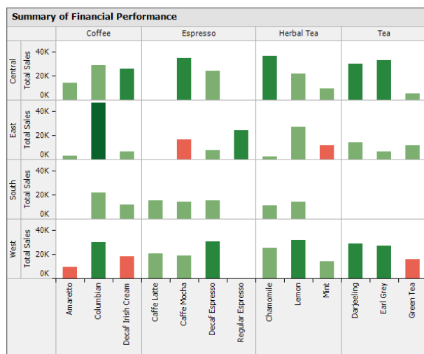
FIGURE I: Visualizing Information
