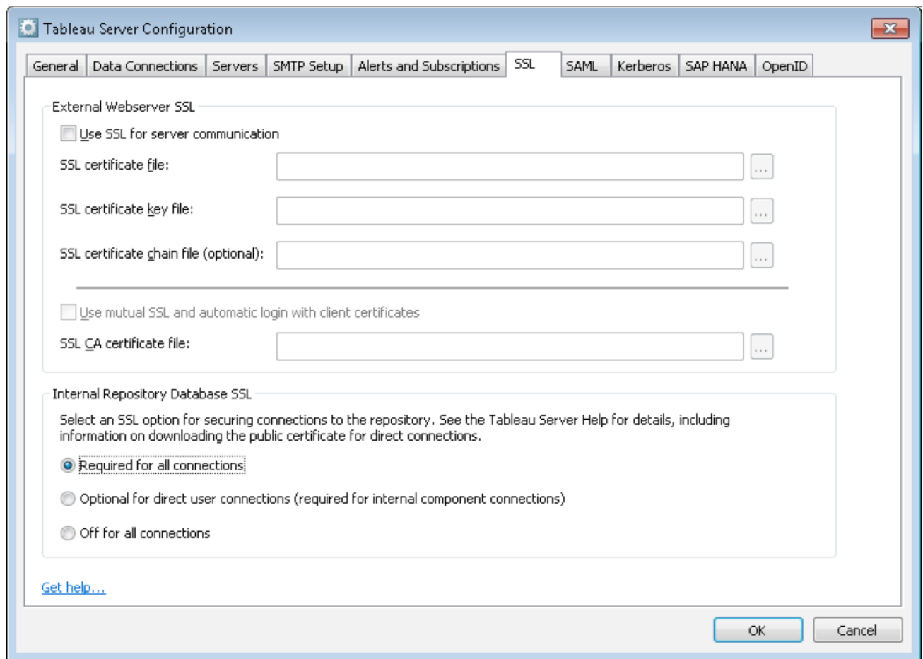
Figure 6. Configuring internal Repository database SSL
