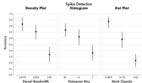
(c) Spike Detection by Visualization
