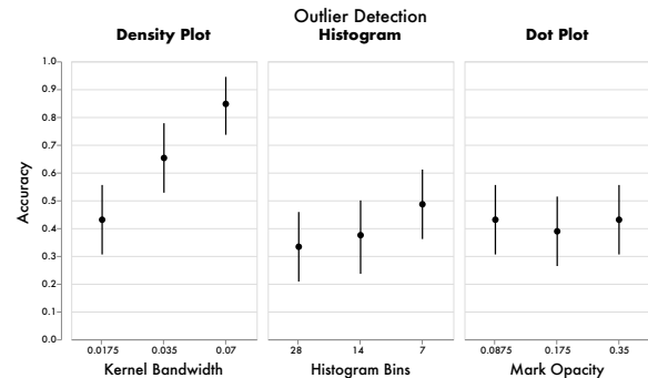
(b) Outlier Detection by Visualization
