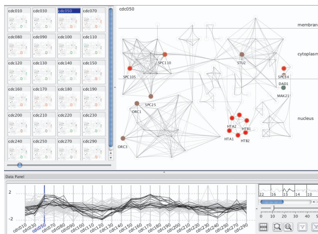
Fig. 6: We set the k-means slider to 10 clusters, and select a cluster of 15 genes that show cyclic behavior.
