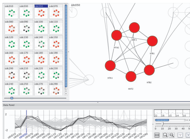
Fig. 7: Selecting the interrelated histone group (HTA1, HTA2, HTB1, HTB2, HHT2) by dragging in the main view shows a clearer pattern of early under-expression in green, then later over-expression in red, in the small multiple views.
