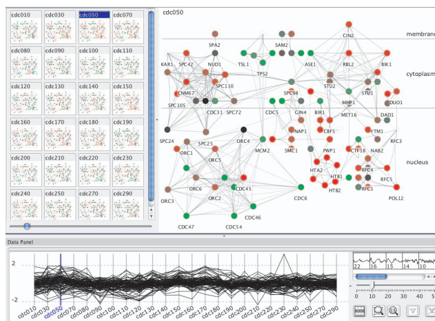
Fig. 5: Initial Cerebral layout of the yeast cell cycle data ( V=104 , E=417 ) shows expression data in a subcellular localized graph context.
